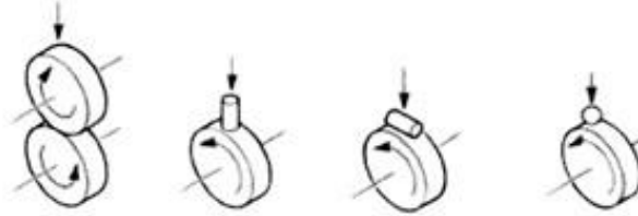
Figure 1. Test configurations of roller-on-roller, roller-on-pin and roller-on-ball.
