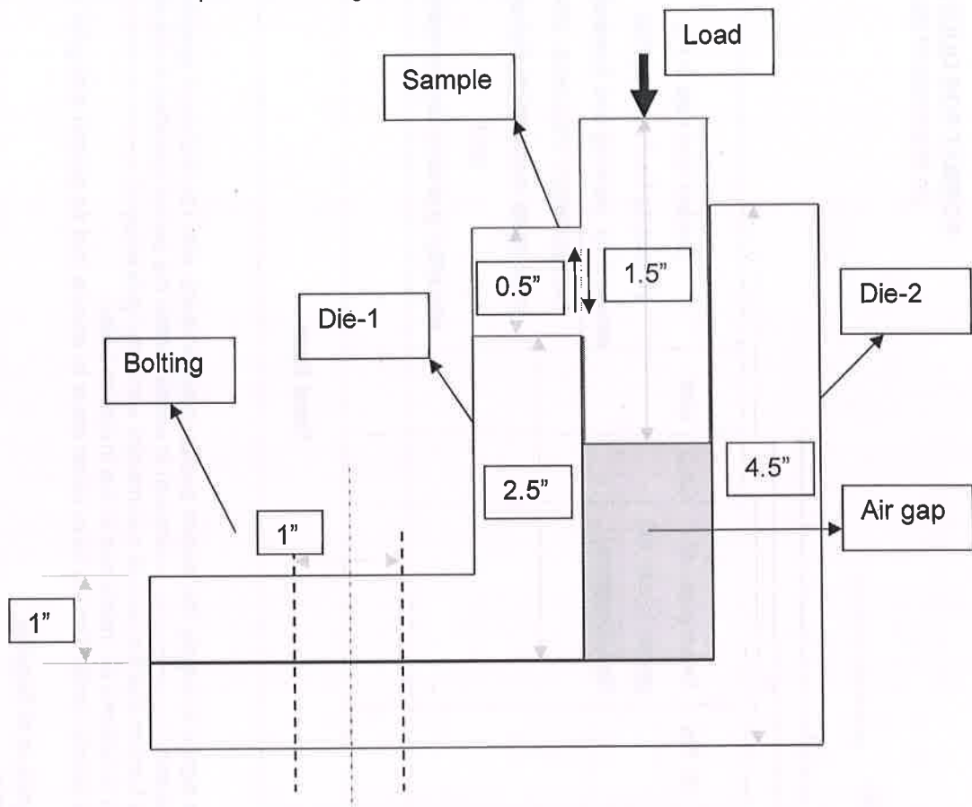
Figure: Shear testing set up
