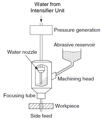
Figure 3. Layout of water jet cutting machine
