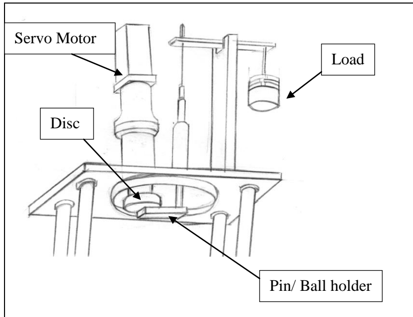
Figure 1. Inverted pin/ball-on-disc set-up.
