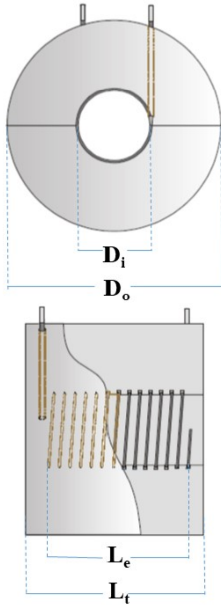
Schematic of heating module
