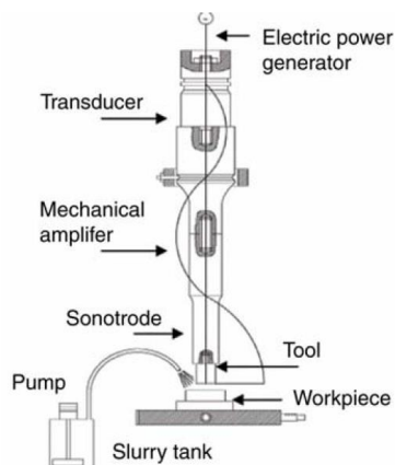
Figure 1. Ultrasonic Machine
