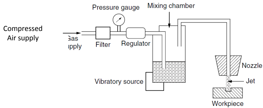
Figure 1. Layout of Abrasive jet Machine
